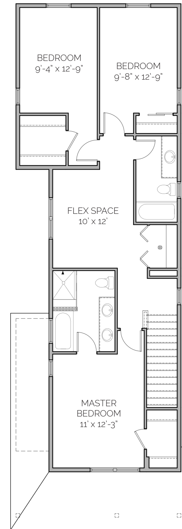
SECOND FLOOR
