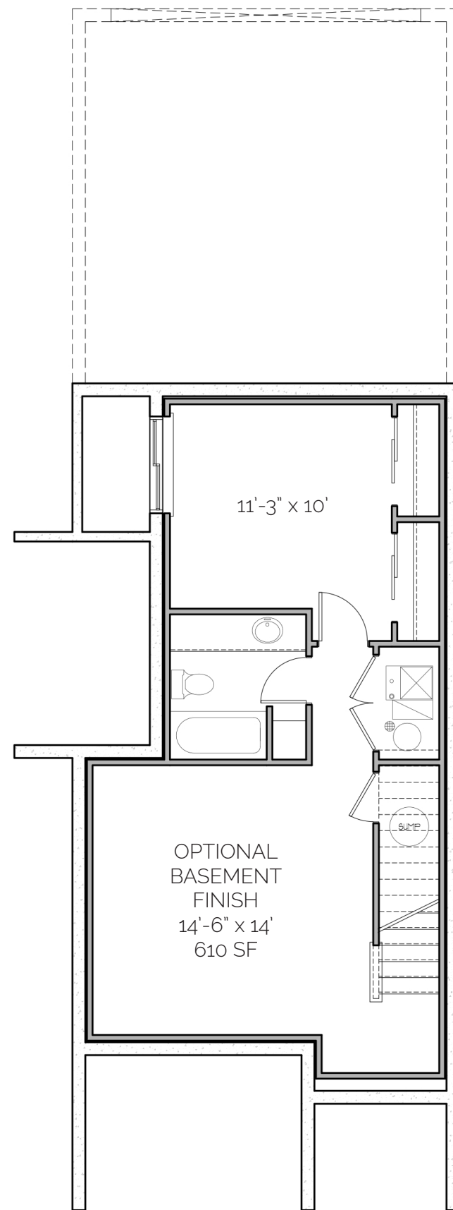
BASEMENT - 639 SF
